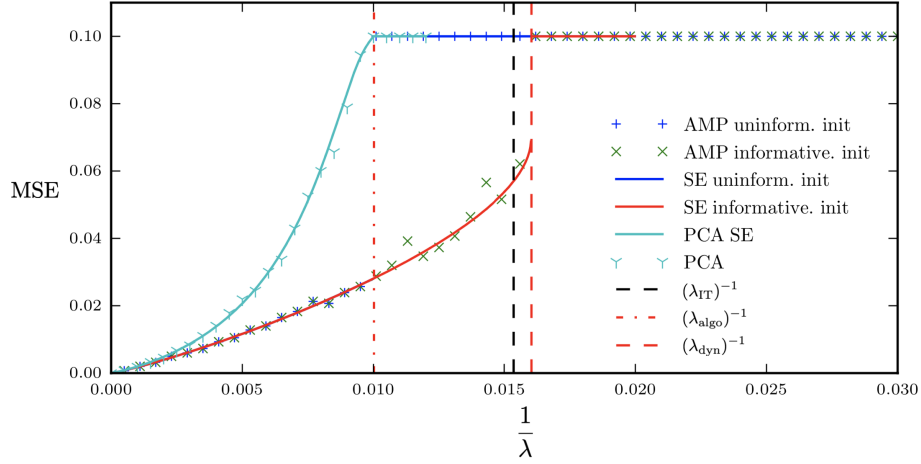
FIGURE 12. Figure from [8]. Comparison between the state evolution and the fixed point of the Low-RAMP algorithm, for the spiked Gauss-Bernoulli model of sparse PCA with rank one and sparsity \rho = 0.1 . The phase transitions stemming from state evolution are 1/\lambda_{\text{algo}} = 0.01 , 1/\lambda_{\text{IT}} = 0.0153 , and 1/\lambda_{\text{dyn}} = 0.0161 . The points are the fixed points of the AMP algorithm run on one typical instance of the problem of size n = 20000 . Blue pluses are the MSE reached from an uninformative initialization q^0 = \varepsilon \ll 1 . Green crosses are the MSE reached from the informative initialization q^0 = \rho .
