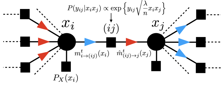
FIGURE 10. Visualization of the messages flowing on a piece of the factor graph for the spiked Wigner model with Rademacher variables. Factors are represented by squares, variable nodes by disks. The hanging factors of connectivity one represent the prior \psi_i(x_i) = P_X(x_i) \propto \delta_{x_i,1} + \delta_{x_i,-1} . From left to right: the variable node i receives factor-to-node messages (red) from its connected factors except the j -th one, i.e., from n - 2 of them. It combines them and spit out a node-to-factor message m_{i \rightarrow (ij)}^t(x_i) (in blue) to factor (ij) representing the compatibility function \psi_{(ij)}(x_i, x_j; y_{ij}) \propto P(y_{ij} | x_i x_j) \propto \exp\{y_{ij} \sqrt{\lambda/n} x_i x_j\} . The factor (ij) then computes the factor-to-node message \hat{m}_{(ij) \rightarrow j}^t(x_j) (red) according to the BP rule and send the result to its next neighbor j . And so forth.
