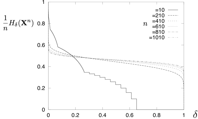
FIGURE 4. From [4]. Convergence of the \delta -essential bit content per bit \frac{1}{n}H(\mathbf{X}^n) for increasing n values, and where X \sim \text{Ber}(p) = 0.1 : we clearly observe that \frac{1}{n}H(\mathbf{X}^n) becomes an increasingly flat function almost independent of \delta (except very close to the border), which constant value tends to H(X) = -0.1 \log_2 0.1 - 0.9 \log_2 0.9 \approx 0.47 bits, except close to the borders \delta = 0 or 1 .
