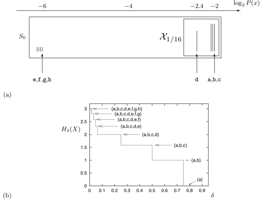
FIGURE 2. From [4]. (a) The outcomes of X ranked by probability. (b) The essential bit content H_\delta(X) . The labels show the smallest sufficient set as a function of \delta . Note H_0(X) = 3 bits and H_{1/16}(X) = 2 bits.
