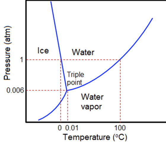
FIGURE 5. Phase diagram of water in the (Pressure, Temperature) plane, the two control parameters in this case, with boundaries delimited by phase transitions.
