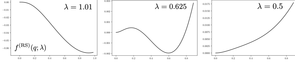
FIGURE 13. Figure from [7]. Plot of the free-energy single-letter potential f^{(\text{RS})}(q; \lambda) as a function of q for different SNR values \lambda . The potential f^{(\text{RS})}(q; \lambda) is the function minimized in (36). Left (easy phase): The SNR is above the algorithmic threshold \lambda_{\text{algo}} = 1 , so AMP yields allows optimal estimation with a MMSE equal to \rho^2 - q_0^2 , where q_0 is the global minimizer of the potential. Optimal estimation being possible at low computational cost this regime is called easy . Middle (hard phase): Below the algorithmic threshold state evolution initialized from q^{t=0} = 0 will remain trapped in the local minimizer of the potential. AMP (as any known efficient algorithm) is therefore sub-optimal. This defines the hard phase . Right (impossible phase): Finally for very low SNR even the MMSE is high ( q_0 is low), so inference is impossible for all algorithms (efficient or not).
