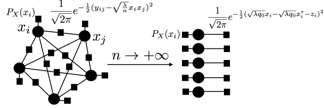
FIGURE 7. Visualization of the decoupling phenomenon happening in the thermodynamic limit: the left model is the original one, the right one is an asymptotically “equivalent” mean-field model with effective Gaussian factors, with SNR related to the minimizer q_0(\lambda, \rho) of the replica symmetric potential.
