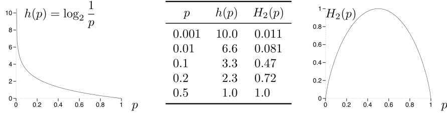
FIGURE 1. From [4]. Information content (in bits as the logarithm is in base 2) of an event with probability p . The less probable an outcome is, the greater its information content. On the right is the binary entropy function H_2(p) , with its maximum at 1/2 .
