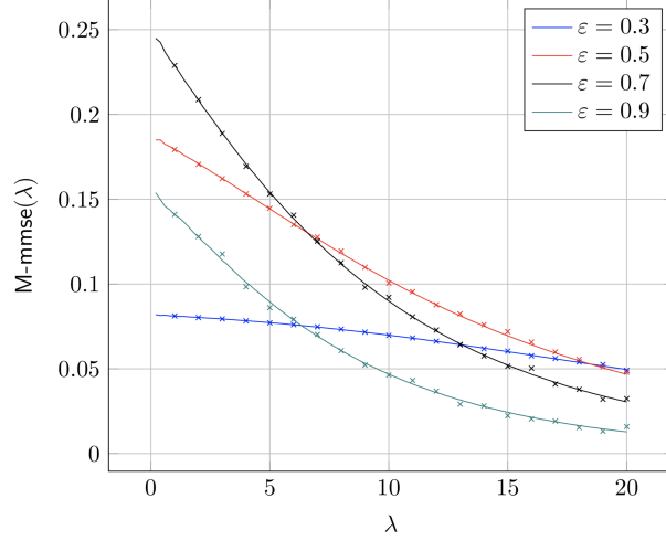
FIGURE 11. Figure from [18]. The solid curves are the state evolution prediction of the asymptotic spike-MSE of AMP \lim_{t \rightarrow \infty} \lim_{n \rightarrow \infty} \text{MSE}_{\text{AMP}}^t for different SNR values \lambda . The crosses mark median MSE incurred by AMP in 100 Monte Carlo runs with n = 2000 for the spiked Wigner model with X_i \sim \text{Ber}(\varepsilon) . In this case there is no hard phase and AMP is always Bayes optimal.
