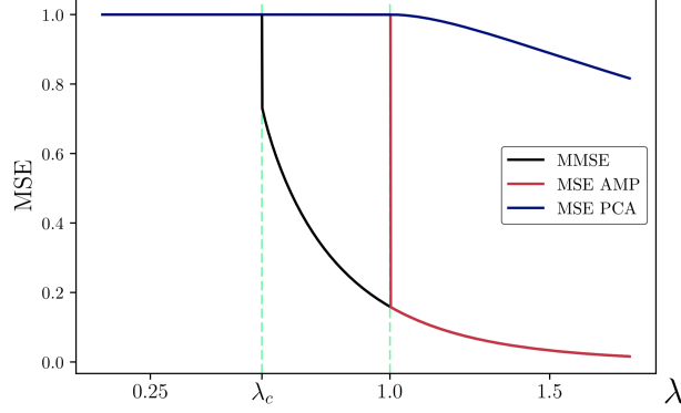
FIGURE 8. Figure from [7]. Plot of the minimum mean-square error given by Corollary 1, the MSE of the approximate message-passing algorithm and of naive PCA for the spiked Wigner model with prior given by (22).
