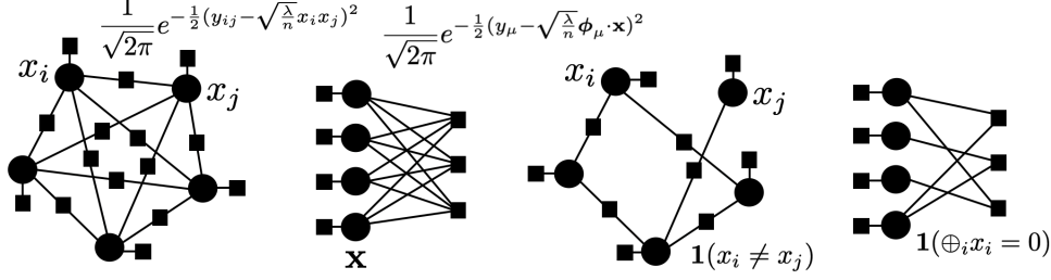
FIGURE 6. Graphical models/factor graphs associated with different inference and combinatorial optimization problems of a mean-field nature (the two first are dense models, the two last are sparse/tree-like). Starting from left: the factor graph of the spiked Wigner model (the factors connected to a single node represent the independent prior contribution P_X(x_i) encoding, e.g., the domain of the variable etc), of high-dimensional linear regression, of the coloring problem, of a low-density parity-check code.
