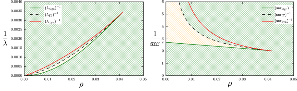
FIGURE 9. From [8]. Phase diagram of the spiked Wigner model with Bernoulli parameters X_i \sim \text{Ber}(\rho) as a function of the sparsity \rho and inverse of the SNR \lambda (left) or the inverse of the total SNR given by \text{snr} := \lambda\rho^2 (right), see (23). There is no phase transition in the system if \rho > 0.04139 and a first order phase transition else. The lower green curve is the algorithmic phase transition of the approximate message-passing algorithm, see section 3, that converges to (\lambda_{\text{algo}})^{-1} = e\rho^2 . The dashed black line is the information theoretic threshold. The upper red curve is the dynamical spinodal where the informative fixed point of state evolution disappears. The orange hashed zone is the hard region in which AMP is sub-optimal (as any known sub-exponential complexity algorithm). In the rest of the phase diagram (green hashed) the AMP provides in the large size limit the Bayesian optimal error.
